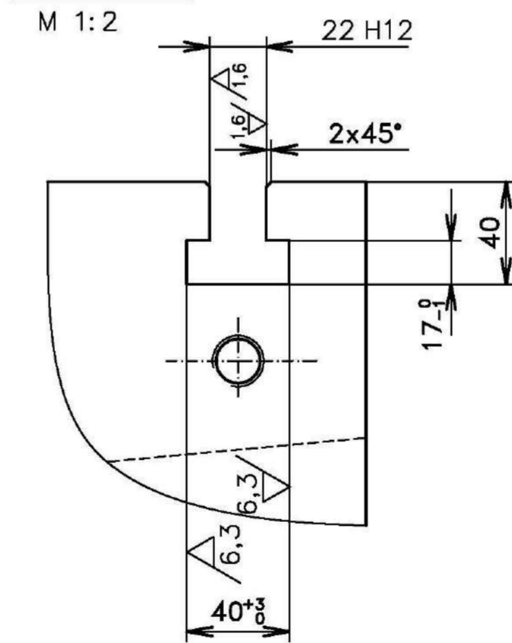
DETAIL D
